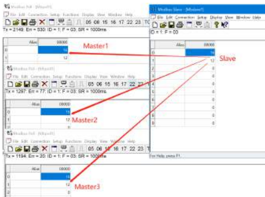
Figure 53. Test result of Modbus multi-host polling
