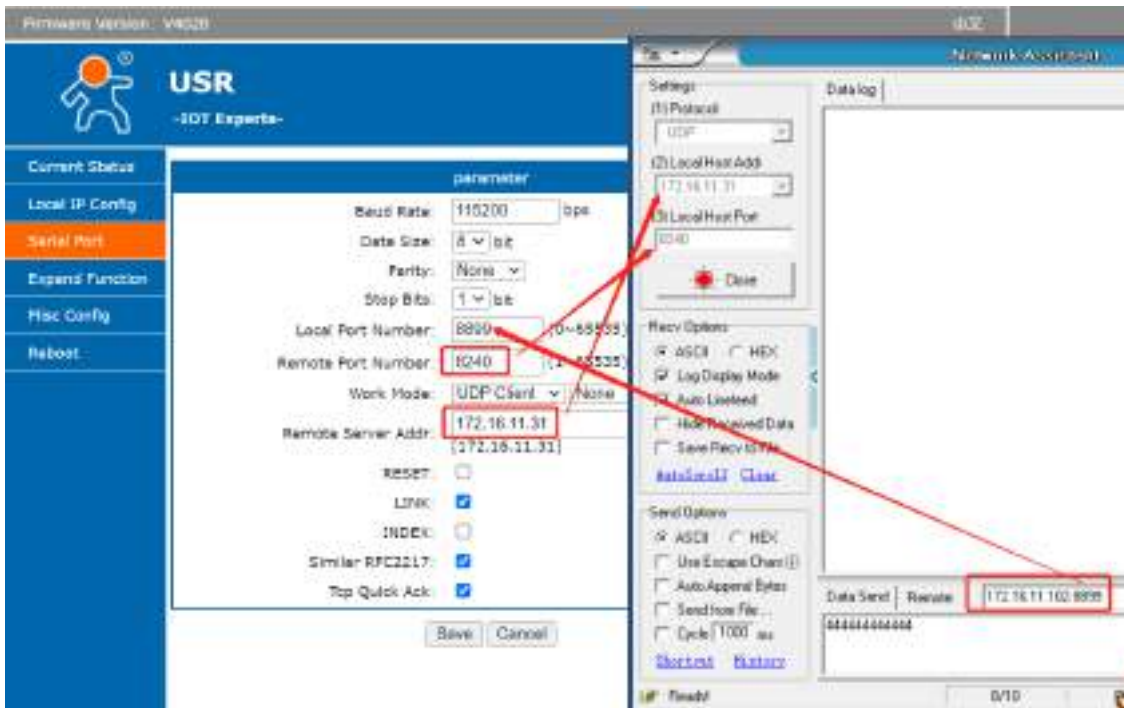
Figure 38. UDP client
